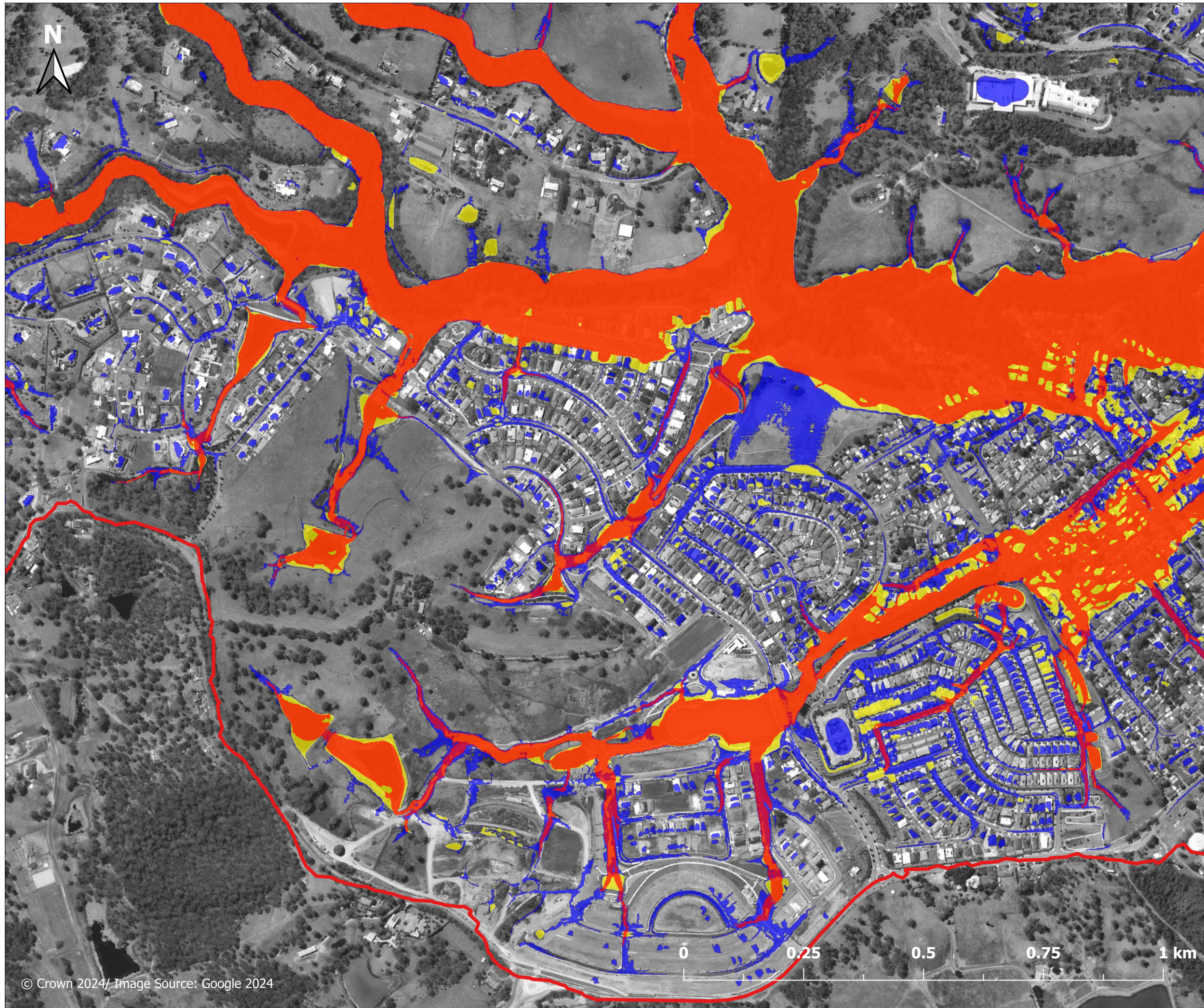
Figure H.2.5.3 Hydraulic categories PMF event West of North Richmond
