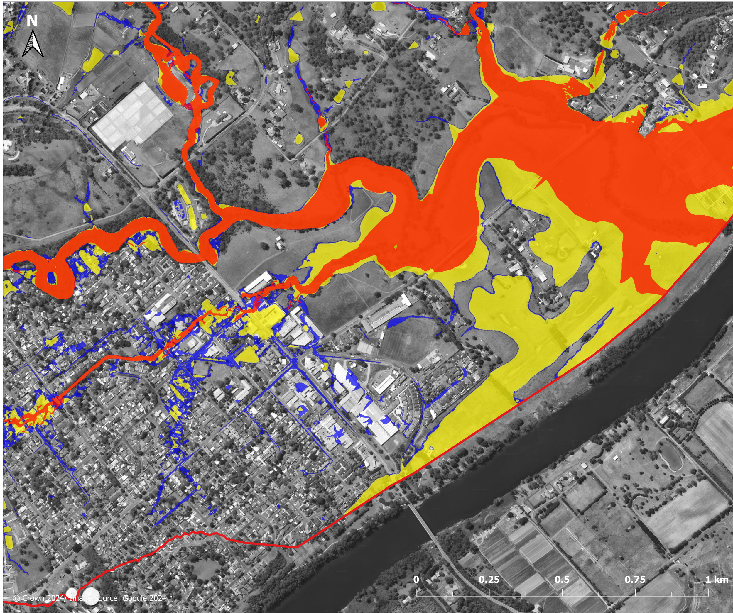
Figure H.2.4.2 Hydraulic categories 1 in 500 AEP event East of North Richmond
