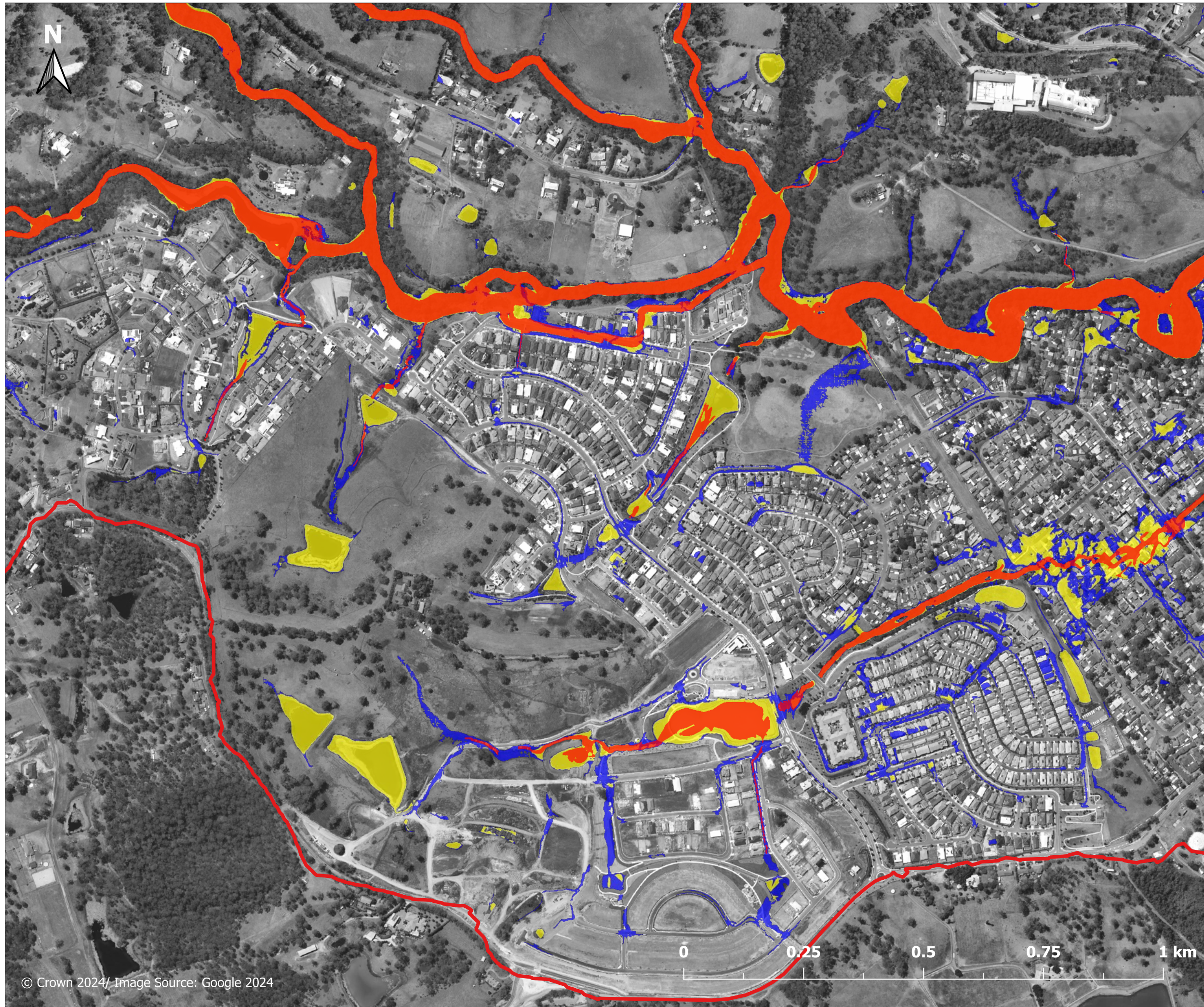
Figure H.2.4.3 Hydraulic categories 1 in 500 AEP event West of North Richmond
