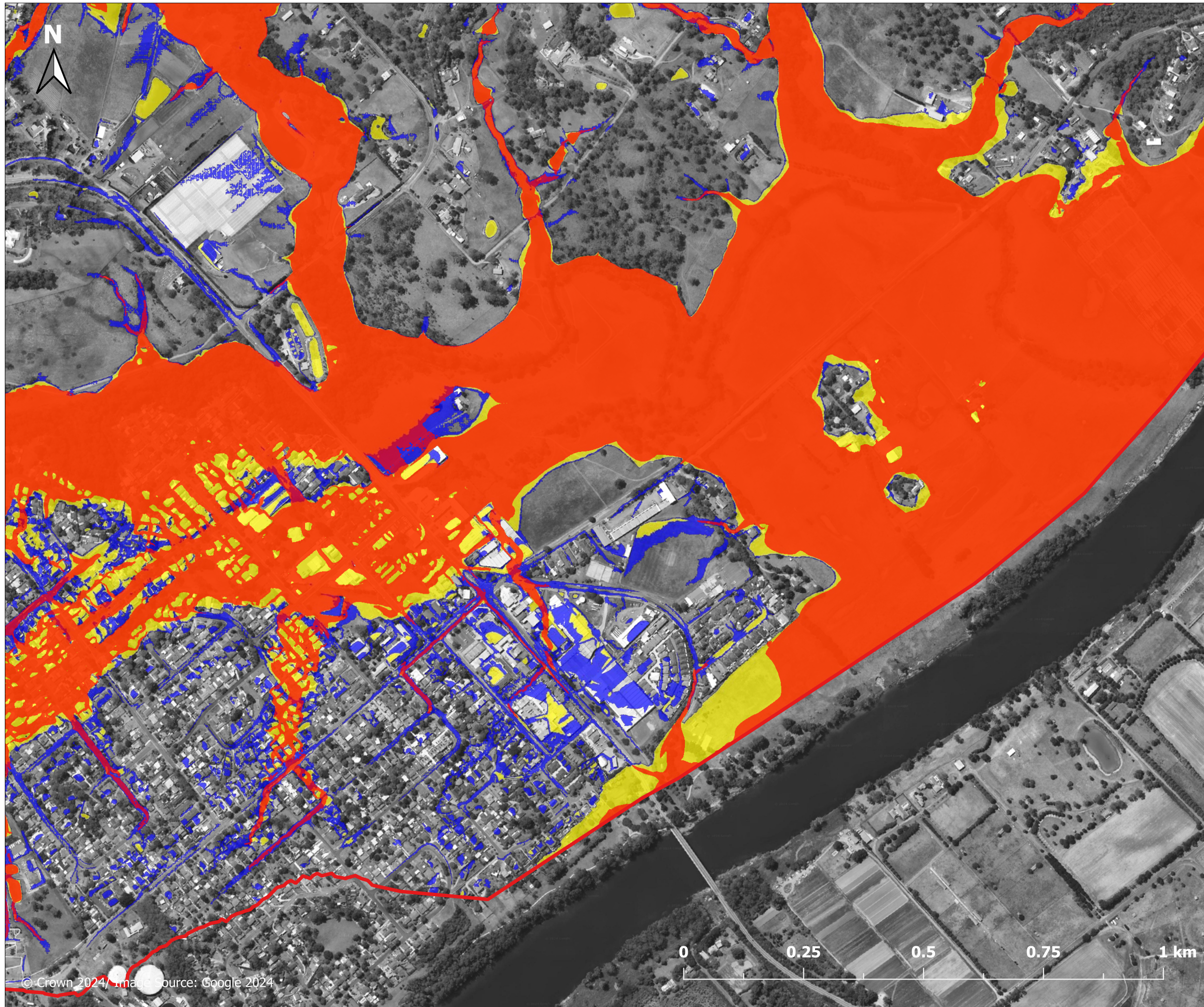
Figure H.2.5.2 Hydraulic categories PMF event East of North Richmond
