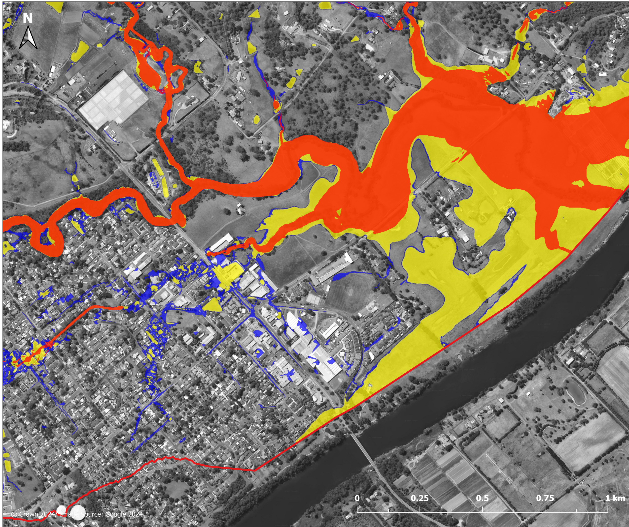
Figure H.2.3.2 Hydraulic categories 1 in 200 AEP event East of North Richmond
